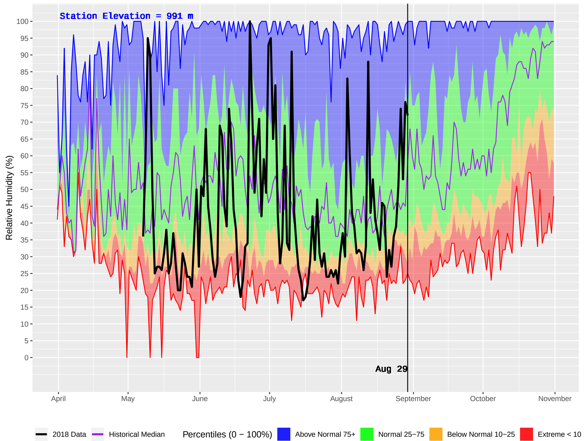
TROUT LAKE (387) : Historical (1987–2016) and Current (2018) Daily Relative Humidity
