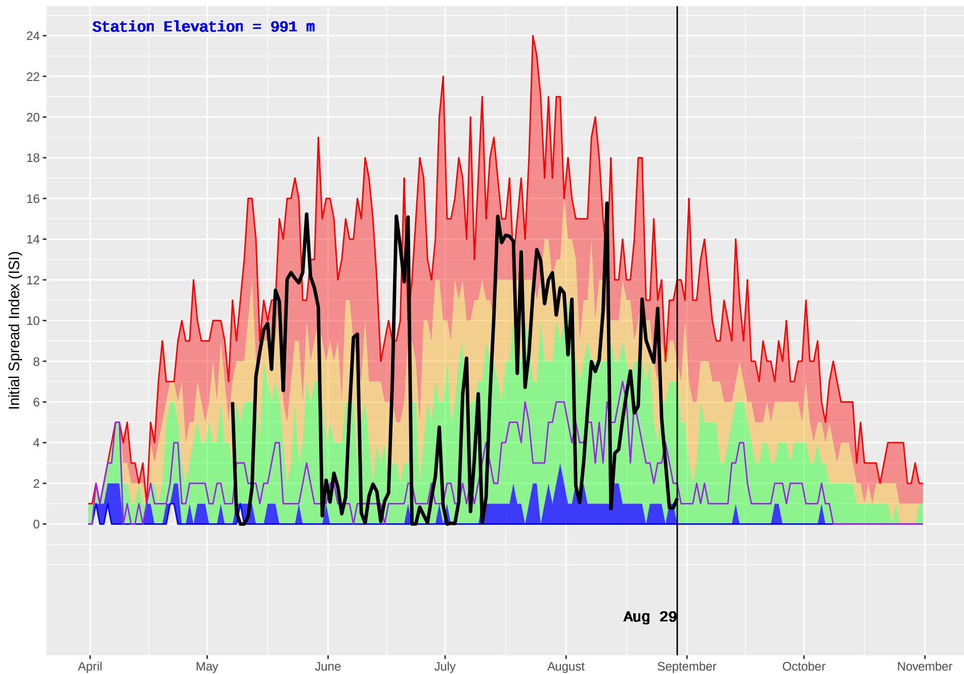
TROUT LAKE (387) : Historical (1987–2016) and Current (2018) Daily Initial Spread Index (ISI)
