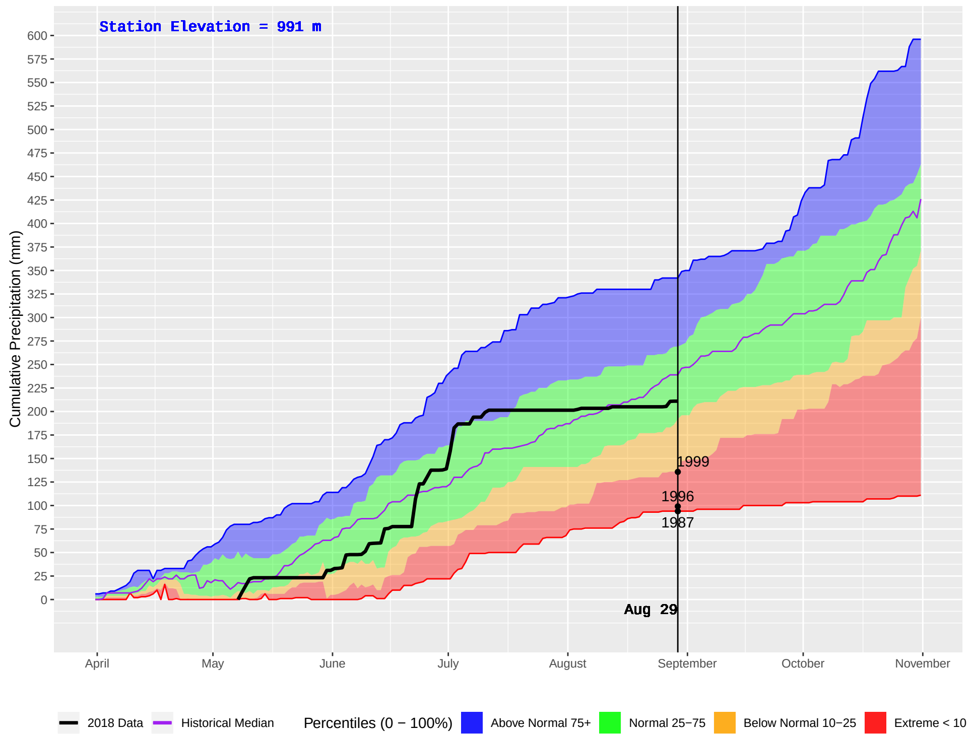
TROUT LAKE (387) : Historical (1987–2016) and Current (2018) Daily Cumulative Precipitation
