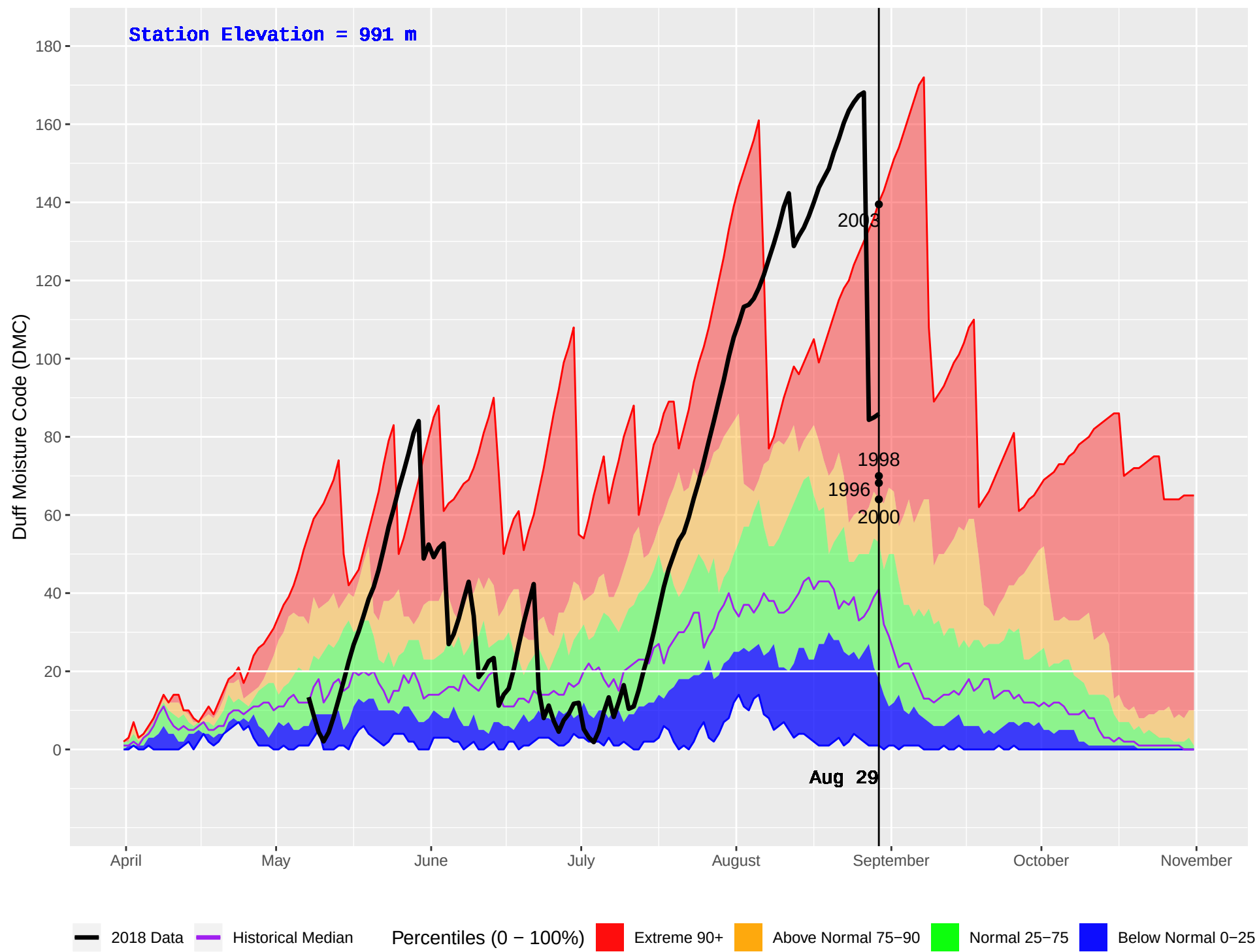
TROUT LAKE (387) : Historical (1987–2016) and Current (2018) Daily Duff Moisture Code (DMC)
