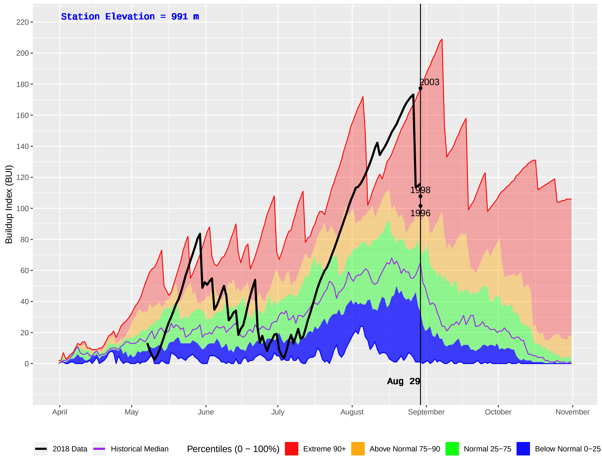
TROUT LAKE (387) : Historical (1987–2016) and Current (2018) Daily Buildup Index (BUI)
