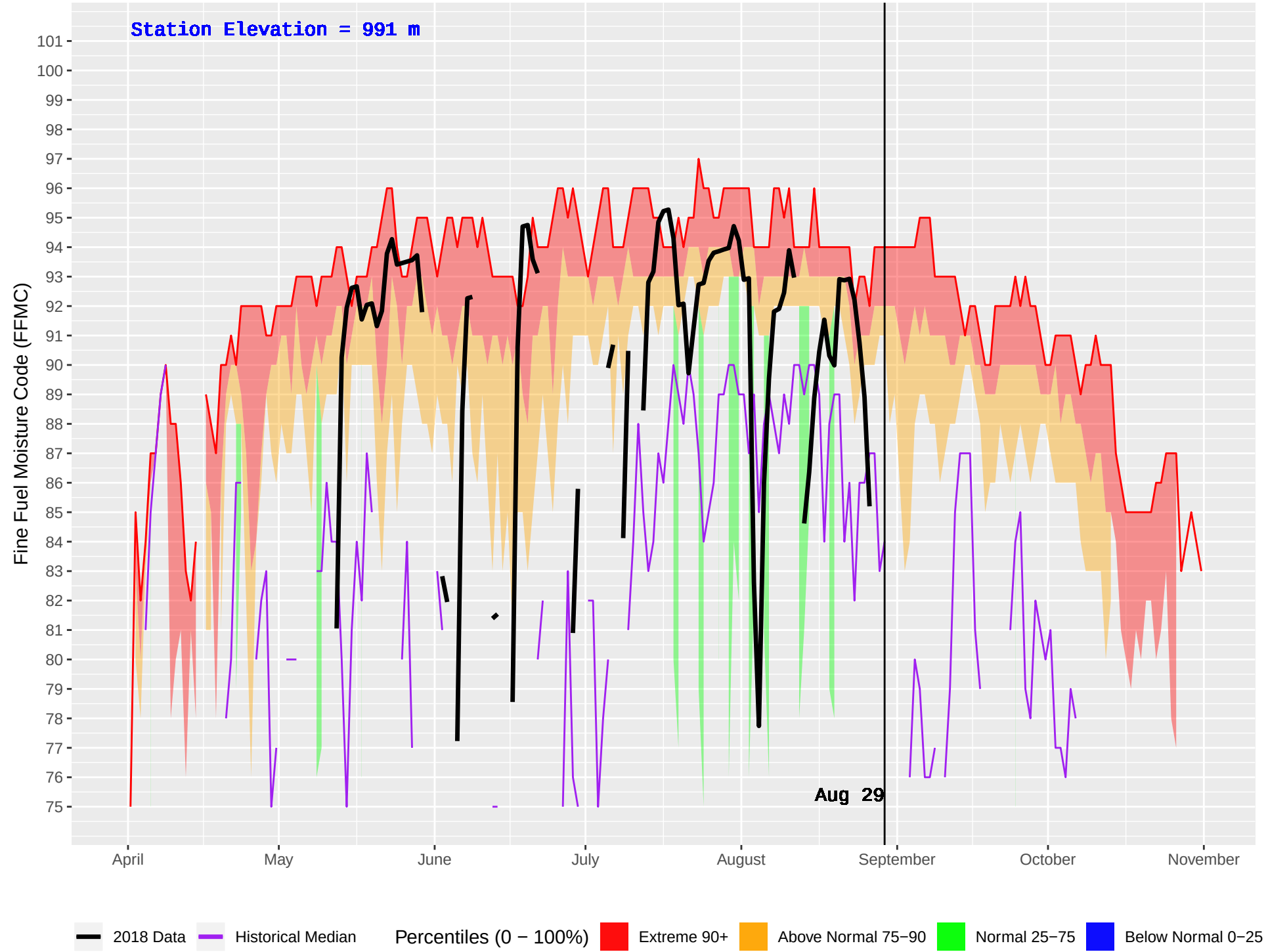
TROUT LAKE (387) : Historical (1987–2016) and Current (2018) Daily Fine Fuel Moisture Code (FFMC)
