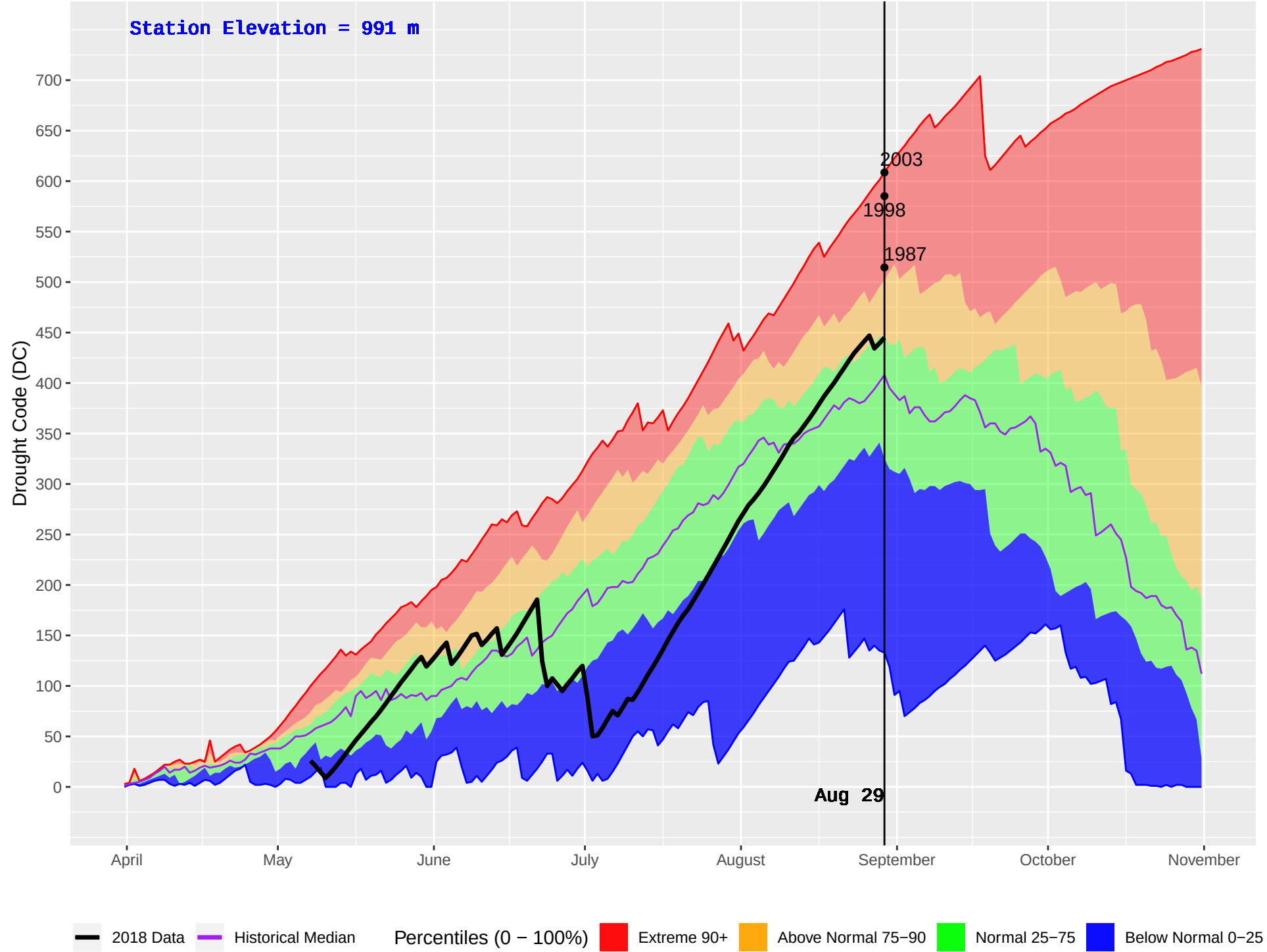
TROUT LAKE (387) : Historical (1987–2016) and Current (2018) Daily Drought Code (DC)
